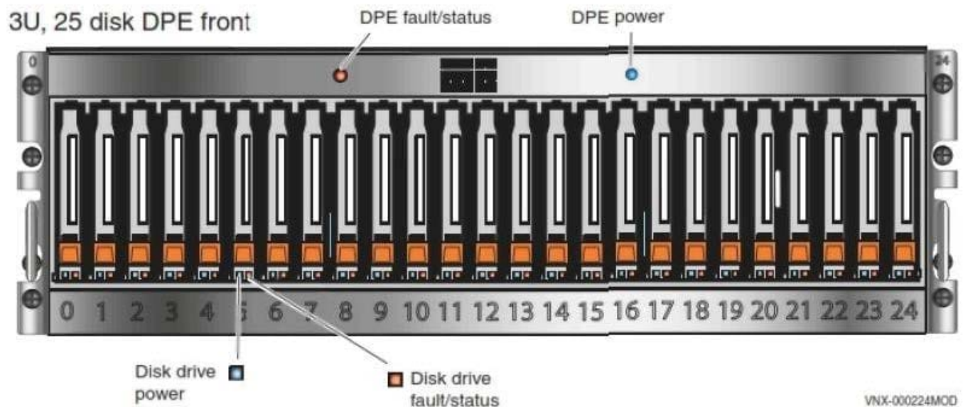
Figure 11 DPE LEDs
